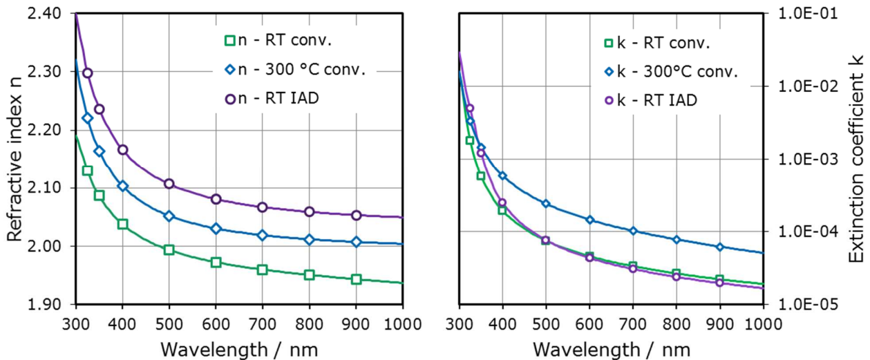
Optical Dispersion
